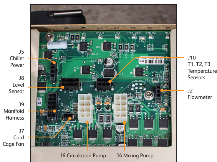
Fig. 8-15 I/O Circuit Card connections
